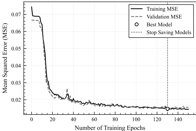
Learning Curve of MHSA-LSTM Model for SolarPlant-2 (Gyeongju)
